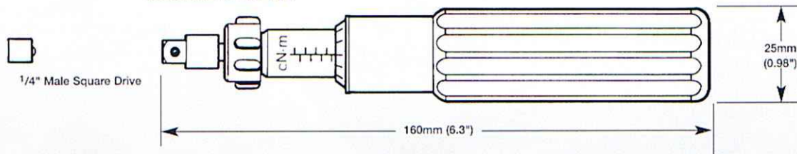
Quickset Minor FH
